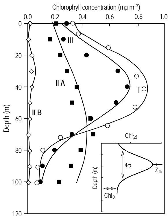
Figure 1. Examples of the chlorophyll concentration ( Chl_z ) profiles with the original data points (symbols) and the representative Gaussian curves for the Yucatan (I), deep-water (IIA and IIB), and Mississippi (III) regions. An idealized deep chlorophyll maximum represented by a Gaussian curve superimposed on a constant background is inserted, showing the parameters.
