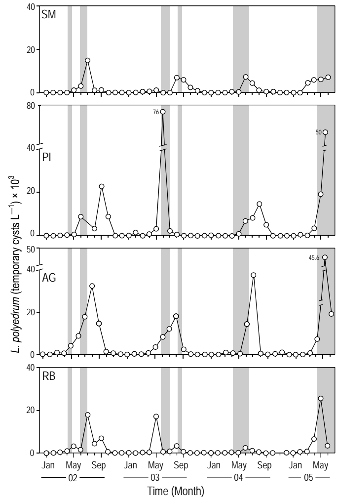
Figure 4. Variability of the abundance of temporary cysts (cysts L^{-1} ) for Lingulodinium polyedrum in the water column at San Miguel (SM), Puerto Interior (PI), Arroyo El Gallo (AG), and Rincón Ballenas (RB) from January 2002 to June 2005. Shaded areas indicate when the abundance of dinoflagellate cells was >10^5 cells L^{-1} during the study period.
